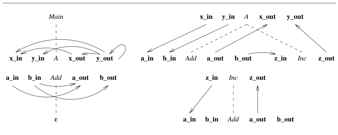
Figure 6. The productions of Figure 5, augmented with attribute dependences.
