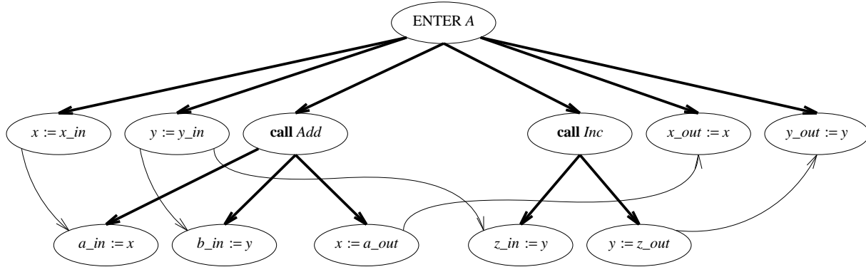
Figure 13. Procedure A 's procedure dependence graph built using interprocedural summary information. The actual-out vertex for argument y of the call to Add has been omitted, and the flow edge from that vertex to the vertex “ z_in := y ” has been replaced by an edge from the vertex “ y := y_in ” to the vertex “ z_in := y ”.
