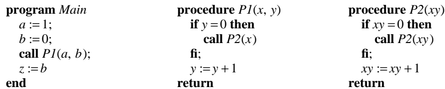
Figure 14. A program with aliasing and the portion of its activation tree needed to compute all alias configurations.
