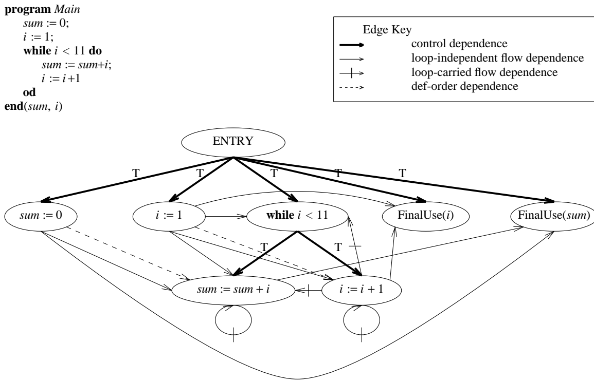
Figure 1. An example program, which sums the integers from 1 to 10 and leaves the result in the variable sum , and its program dependence graph. The boldface arrows represent control dependence edges, solid arrows represent loop-independent flow dependence edges, solid arrows with a hash mark represent loop-carried flow dependence edges, and dashed arrows represent def-order dependence edges.
