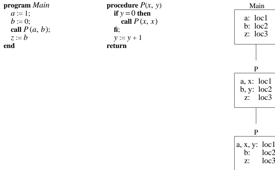
Figure 14. A program with aliasing and the portion of its activation tree needed to compute all alias configurations.
