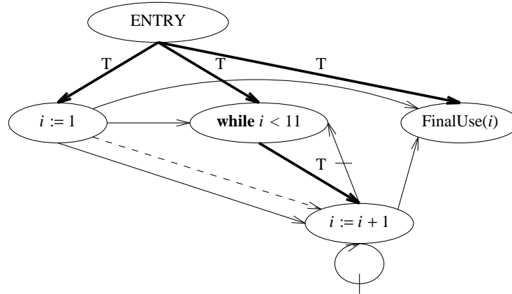
Figure 3. The graph and the corresponding program that result from slicing the program dependence graph from Figure 1 with respect to the final-use vertex for i .
