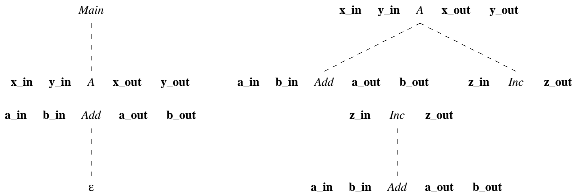
Figure 5. The productions of the example linkage grammar shown in tree form. Each nonterminal is annotated with its attributes; a nonterminal's inherited attributes are placed to its left; its synthesized attributes are placed to its right.
